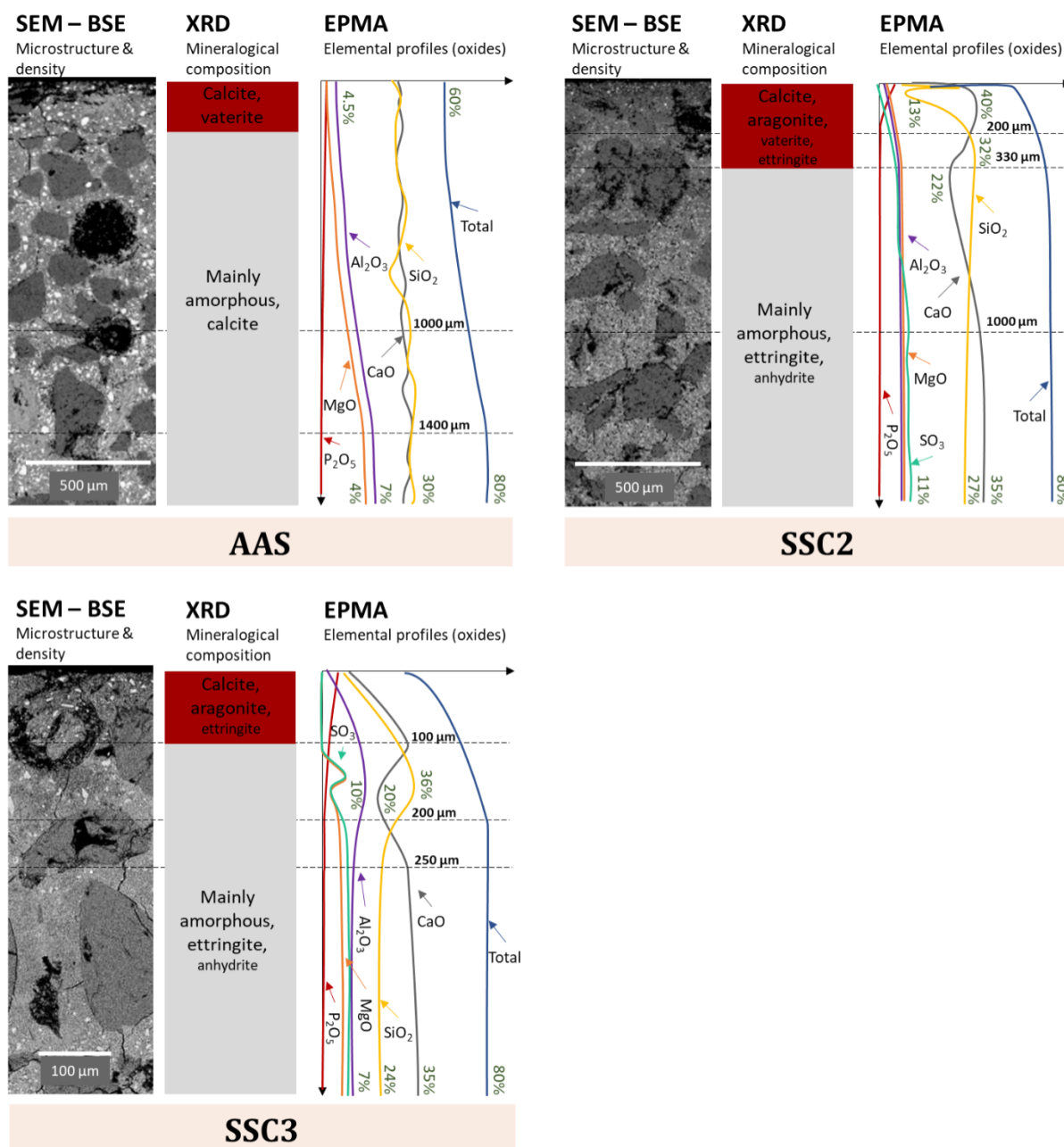
Figure 7. BSE-SEM images and mineralogical and chemical compositions of the different zones of the AAS, SSC2 and SSC3 mortars after 2 years and 3 months of exposure in the liquid phase of a digester
