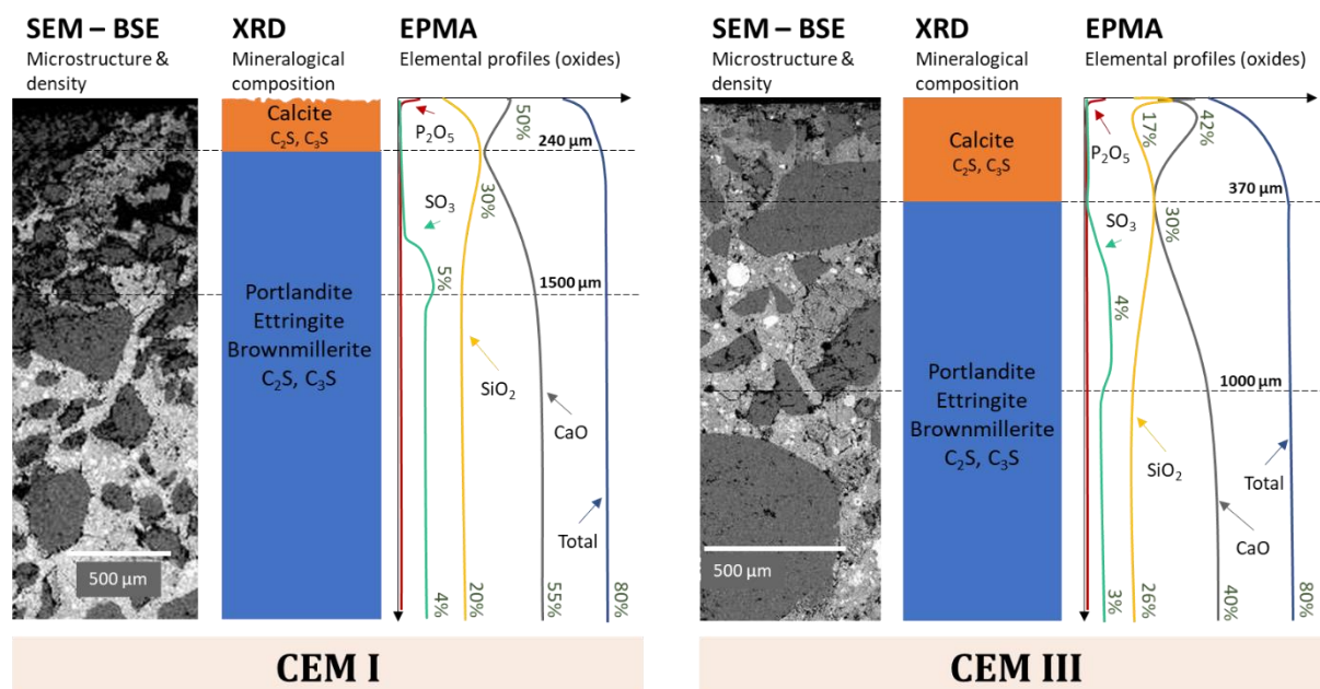
Figure 5. BSE-SEM images and mineralogical and chemical compositions of the different zones of the CEM I and CEM III mortars after 2 years and 3 months of exposure in the liquid phase of a digester
