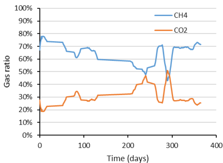
Figure 3. CH 4 and CO 2 ratio (compared to the total amount of CH 4 and CO 2 ) in the gas phase of the digester between March 2019 and March 2020
