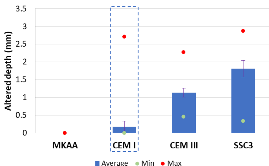
Figure 8. Performance ranking of the mortars according to their altered depth after 1 year and 10 months of exposure to the gas phase of the digester – blue dashed frame corresponds to the CEM I-based reference mortar
