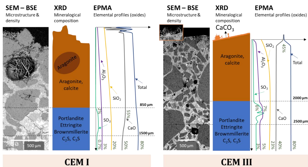
Figure 9. BSE-SEM images and mineralogical and chemical compositions of the different zones of the CEM I and CEM III mortars after 1 year and 10 months in the gas phase of a digester
