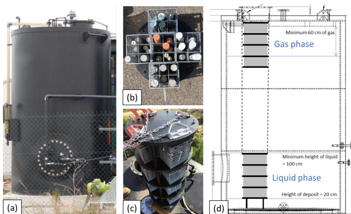
Figure 1. (a) Semi industrial scale digester used for the in-situ exposure – SOLIDIA, Bélèsta-en-Lauragais, (b) samples compartmented in dishwasher baskets, (c) assembly of the baskets on a polypropylene structure, and (d) positioning of the basket structures in the digester
