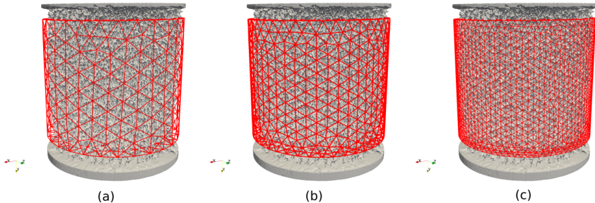
Fig. 5 Three finite element mesoscale DVC discretizations. (a) 33 voxels, (b) 23 voxels and (c) 12 voxels.
