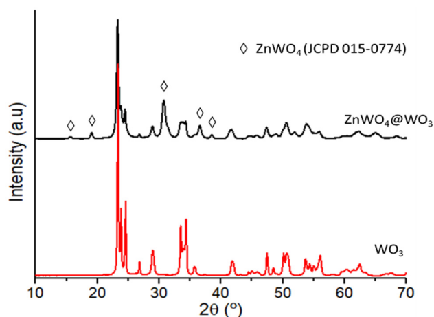
Figure 16. XRD analyses of the composite \text{ZnO}@\text{WO}_3 \cdot \text{H}_2\text{O} (0.5 equiv. \text{Zn}(\text{Cy})_2 ) annealed at 500^\circ\text{C} in air. The diffraction peaks correspond to the well crystallized \text{WO}_3 monoclinic phase. The peaks corresponding to the additional \text{ZnWO}_4 phase are marked with a diamond.
