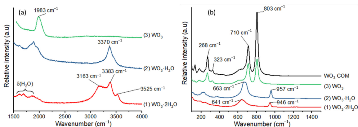
Figure 5. Raman spectra of (1), (2) and (3) (a) in the range 1500–4000 cm −1 and (b) in the range 100–1500 cm −1 .
