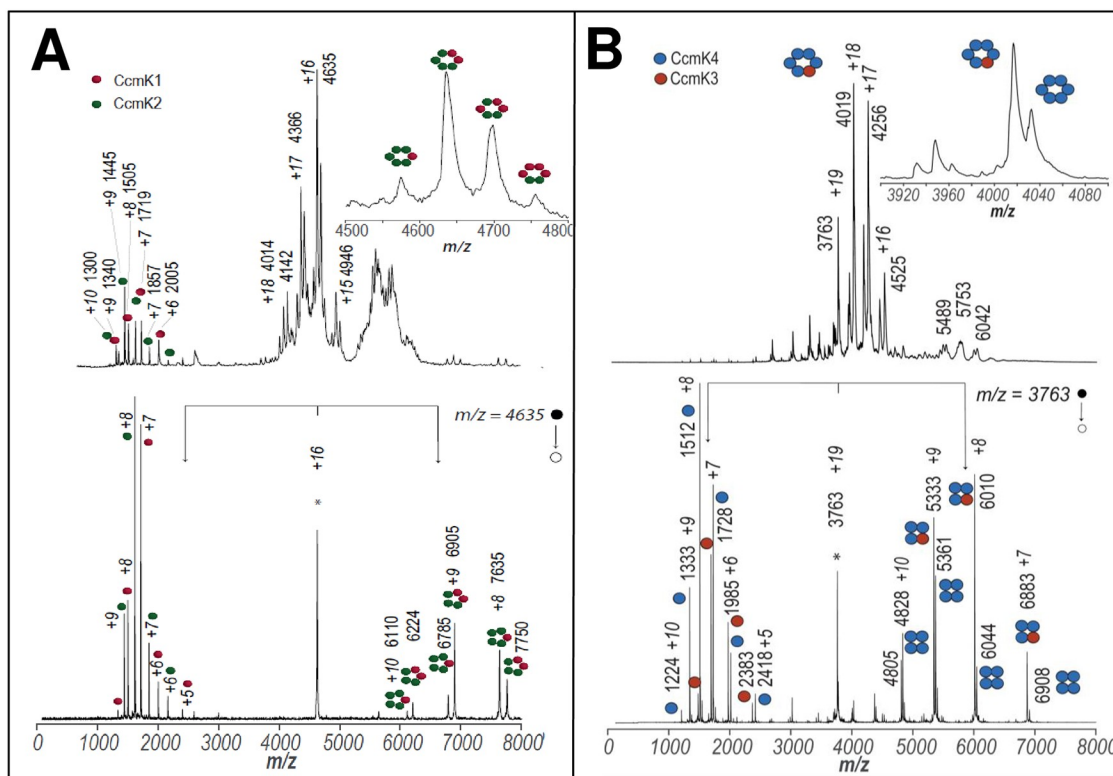
Fig 2. Hetero-hexamer characterization by native mass spectrometry. A, Spectra recorded on fractions purified from cells co-expressing CcmK1-His 4 together with CcmK2-FLAG; B, similarly, but from cells co-expressing His 4 -CcmK4 and CcmK3-FLAG. Positive-ion mode native ESI-MS spectra are presented on top panels. These spectra are dominated by signals from multiply charged ions of hexamers. Potential higher order assemblies were observed in combinations with CcmK2. Bottom panels present an example of MS-MS collisional activation data collected on hexamer precursor ions selected from top spectra (indicated with an asterisk). An asymmetric charge partitioning is noticed, hexamers dissociation resulting in two type of monomers and either pentameric species with CcmK1/K2 (left) or tetrameric species with CcmK3/K4 (right). Monomer masses permitted to attribute picks to either CcmK1 (red spheres), CcmK2 (green), CcmK3 (orange) or CcmK4 (violet). Species m/z values and charges are indicated for major peaks. Cartoons schematically illustrate the stoichiometries of detected protein complexes and subcomplexes. Molecular weights of neutral species estimated from data from different charge states are compiled in S1 Table . Please notice that tags were removed prior to spraying by treatments with TEV protease.
