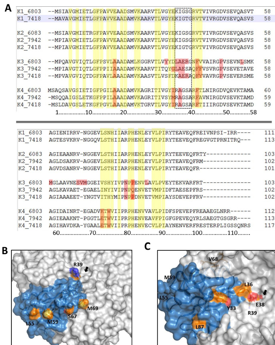
Fig 4. Sequence and structural considerations on CcmK3 paralogs. A, Sequence alignment of sequences of CcmK from Syn6803 , Syn7942 and Hal7418 . Residues directly participating in inter-monomer contacts in 3D structures of homo-hexamers are shaded in yellow. In red are highlighted notable substitutions present in Syn6803 CcmK3, which differ considerably in other paralogs and can be shared or not by CcmK3 in other species. The rectangle contoured by discontinuous traces indicate residues that line central CcmK hexamer pores. B, C Presumed localization of some notable residue substitutions in the CcmK3 Syn6803 structure furnished by SWISS-MODEL (CcmK3_1 in the main text), when compared to other CcmK. The surface and ribbon representation are shown with one chain colored light blue, neighbor subunits in grey. Panel B presents the water-exposed orientation of several hydrophobic side-chains residues localized on the predicted \alpha -helix-2 of CcmK3 (balls and sticks representation, with carbon atoms in orange, nitrogens in blue, oxygens red and sulfur atoms in yellow), as well as Glu38-Arg39 residues lining the central hole. The helix runs from the hexamer edge to the center, and is followed by the stretch comprising S67 to M69, where a residue insertion specific of Syn6803 CcmK3 occurs. The emplacement of the hexamer clogged central hole is indicated by the arrow. The model is viewed from the convex face. Panel C shows the emplacement of other diverging residues, like the Tyr33, the Leu87 or the pore-clogging Glu38-Arg39 residues. The hexamer model is viewed from the concave face and the emplacement of the clogged central pore is indicated by the arrow. Please notice that the side-chains of Arg39, Leu55, Met59 and Val68 lie on the opposite face.
