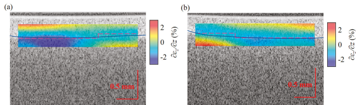
Figure 7. Strain-gradient of \varepsilon_z in the z -direction. (a,b) are 2D strain-gradient maps of the cross-section (c-i) and (c-ii) in Figure 6 respectively plotted on their 2D OCT cross-sectional images. The purple dashed line and blue solid line indicate the estimated interface and physical interface of the two layers respectively.
