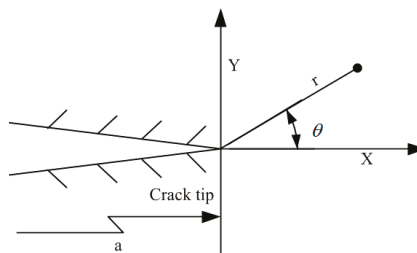
Figure 2. Coordinate system around a crack tip.
