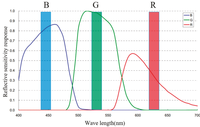
Figure 1. Quantum efficiency of the color camera.
