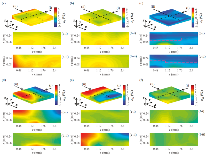
Figure 6. 3D strain fields of a double-layer phantom under compression. (a–c) Normal strains in the x , y and z directions respectively. The purple dashed lines in (c-i) and (c-ii) indicate the interface of the two layers. Two strain maps shown underneath each of the 3D displays are the images of the cross-sections along the dashed lines.
