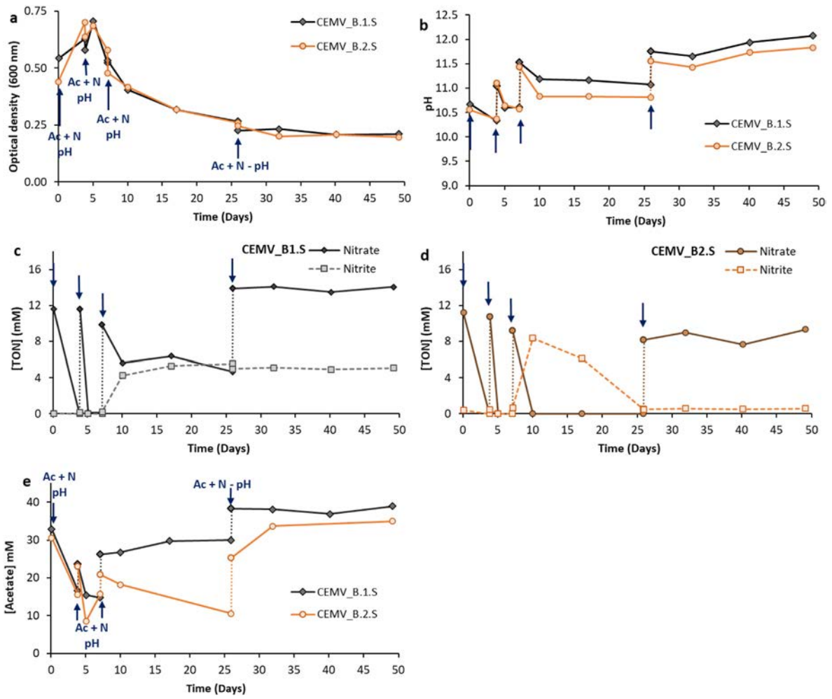
Fig. 7. Evolution of bacterial growth (a), the pH (b), nitrate and nitrite concentrations for the supernatant collected at the end of the second set of experimentations with cement paste immersed during 55 days i.e. the reactor CEMV B1.S (c) and the reactor CEMV B2.S (d), the acetate concentration (e) for the reactor CEMV B1.S (black) and the reactor CEMV B2.S (orange) without cement paste - N nitrate addition, N + A nitrate and acetate addition, pH pH adjustment. (For interpretation of the references to colour in this figure legend, the reader is referred to the Web version of this article.)
