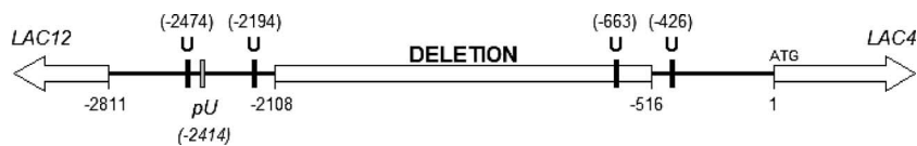
FIG. 5. Deletion identified in the LAC12 - LAC4 intergenic region of the plasmid isolated from the evolved strain (T1-E). The 1,593-bp deletion (open box) was mapped between positions -516 and -2108, +1 referring to the adenosine in the LAC4 initiation codon. The functional UAS elements (U) present in the LAC promoter (13) are represented by vertical black bars and correspond to the 17-bp consensus sequence 5'-CGG(N5)A/T(N5)CCG-3' (in the figure, the central position of the consensus sequence at each UAS is indicated in parentheses). The gray vertical bar represents an additional putative UAS ( pU ) found in T1 and T1-E (see the text for details).
