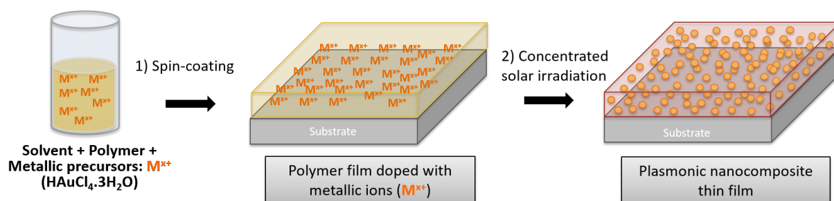
Figure 1: Main steps of the fabrication of plasmonic nanocomposites under concentrated solar irradiation
