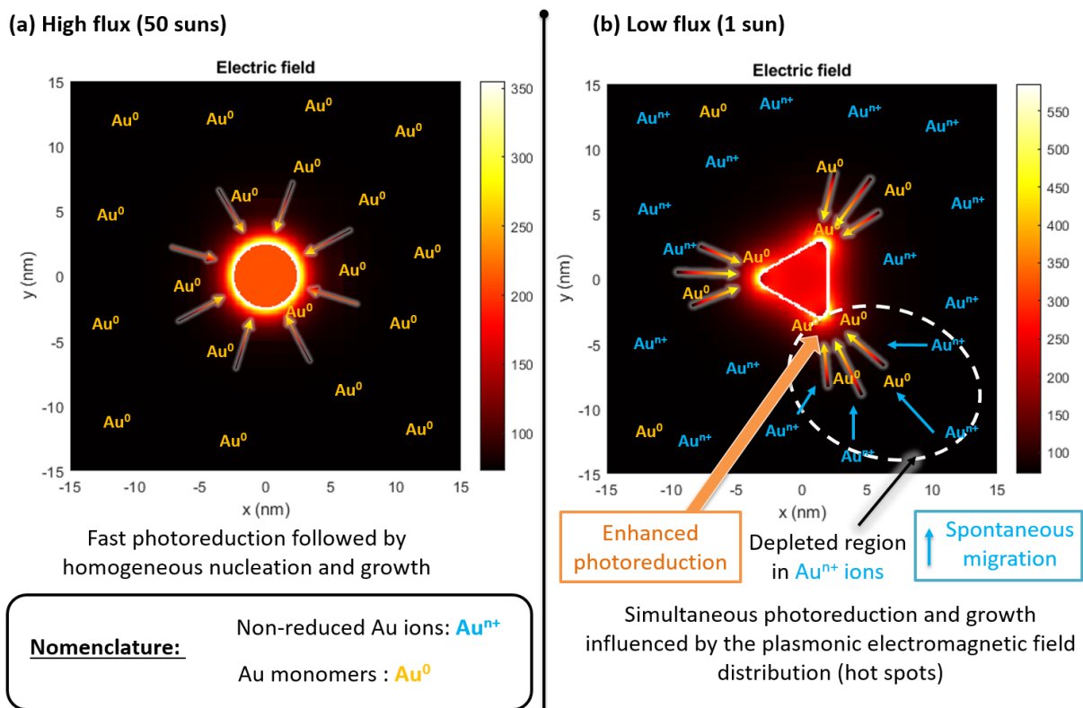
Figure 9: Scattered field map for (a) a nanospheres and (b) a nanoprism under non-polarized light along with schematic illustrations of possible growth mechanisms: Homogenous nucleation and growth at high flux in (a) and anisotropic growth induced by plasmonic hot spots in (b).
