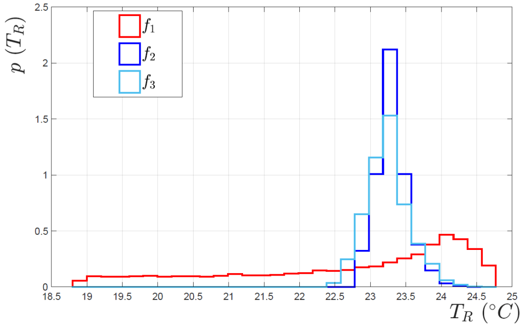
Fig.12: Probability density function of T_R obtained with the 3 different cost functions ( R_P = 0.3 ; R_S = 1 and N = 25 )
