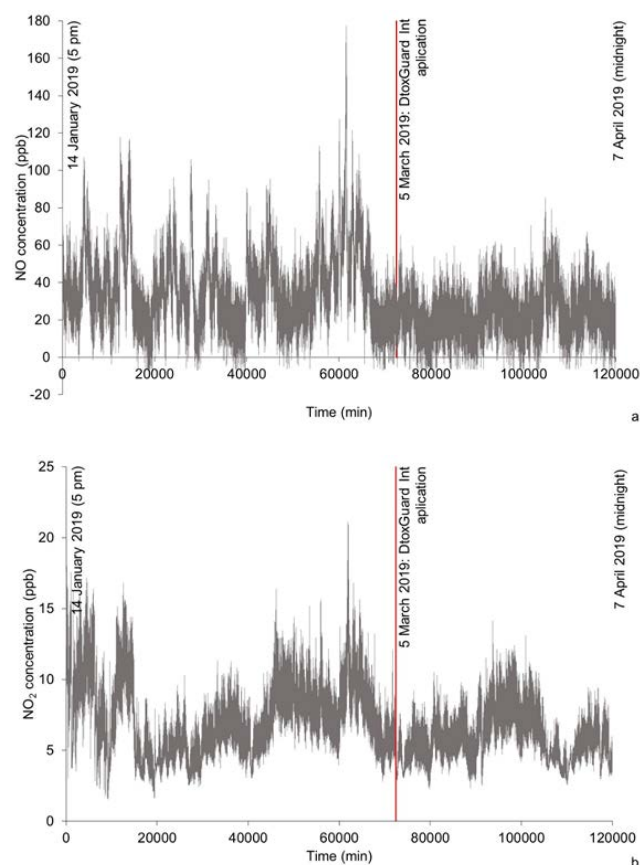
Figure 5. (a) NO indoor concentrations; (b) NO 2 indoor concentrations. The DtoGuard ® Int coating was applied to the wall on the 5 th of March 2019. Notice the different scales
