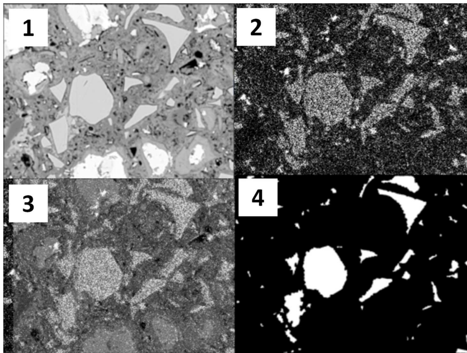
Figure 2. The steps applied in measurement of the degree of slag reaction using SEM-EDX methods: (1) SEM image, (2) Mg-EDS Mapping, (3) Superimposition of BSE and EDS images and (4) Identification of the GGBS particulates (unreacted).
