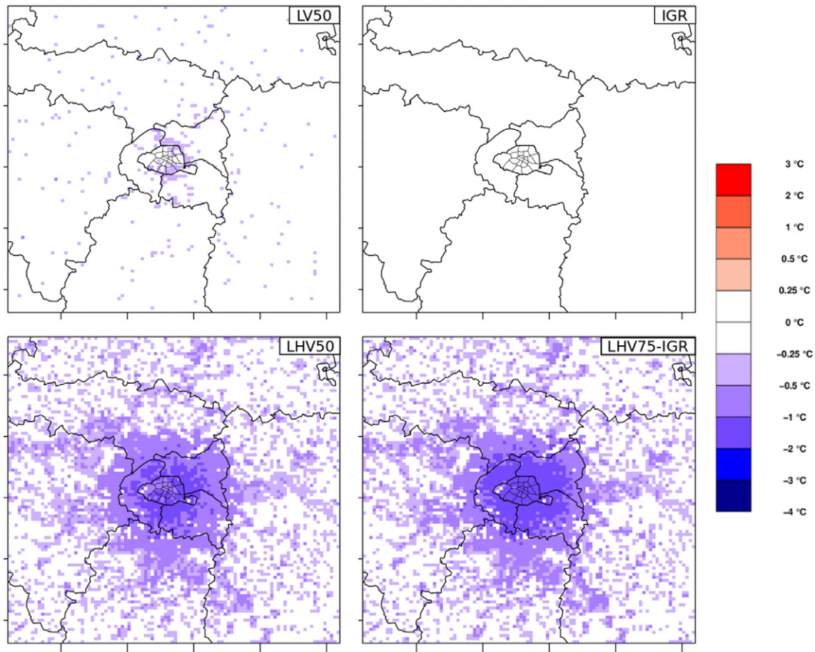
Fig. 3. Spatial distribution of the impacts of greening over minimum daily urban 2m-temperatures for intermediate ground greening (LV50 and LHV50), roof greening (IGR) and maximum greening (LHV75-IGR), expressed as the average impacts during the six days of the heat wave.
