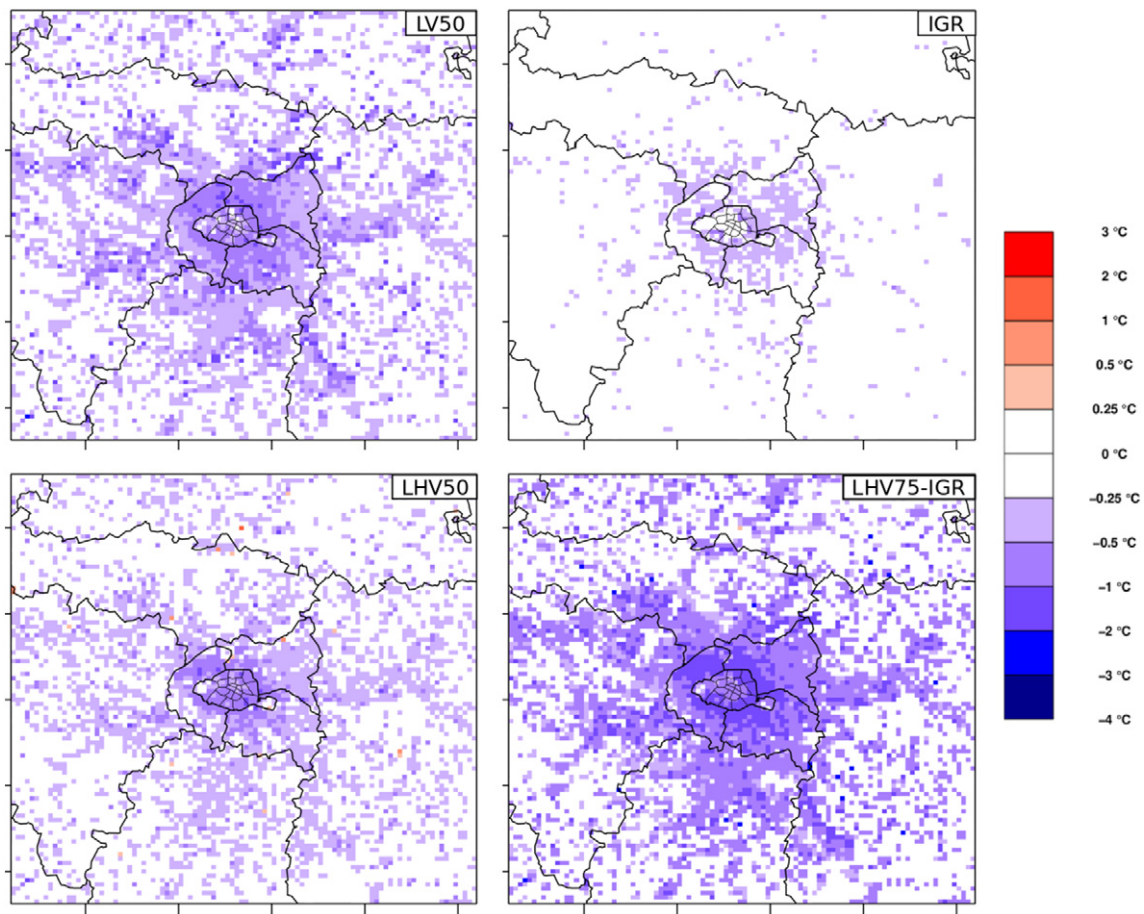
Fig. 4. Spatial distribution of the impacts of greening over maximum daily urban 2m-temperatures for intermediate ground greening (LV50 and LHV50), roof greening (IGR) and maximum greening (LHV75-IGR), expressed as the average impacts during the six days of the heat wave.
