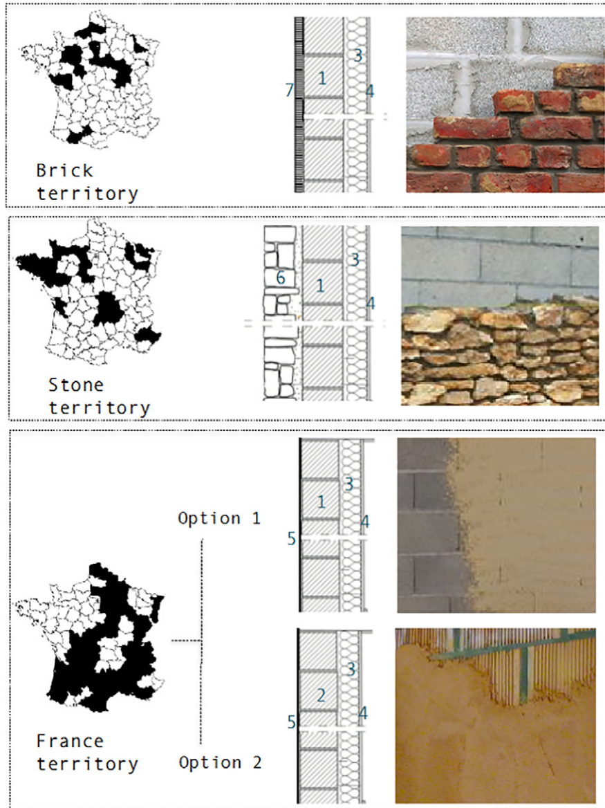
Fig. 5. Constructive system for the walls for the example of low-rise residential buildings of construction period P5. Information is provided on the main material, the internal and external coating as well as the insulation material.
