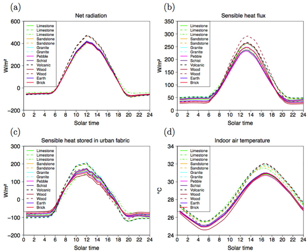
Fig. 6. Sensitivity of the diurnal cycle of the urban surface energy balance on the main wall material and the roof covering material. (a): net radiation, (b): sensible heat flux, (c): storage heat flux and (d): indoor air temperature. The results are averaged over June, July, August (JJA). The continuous lines depict the buildings with a roof covered by tile-brick, the dashed (dash-dotted) lines the buildings with a roof covered by slate (Zinc).
