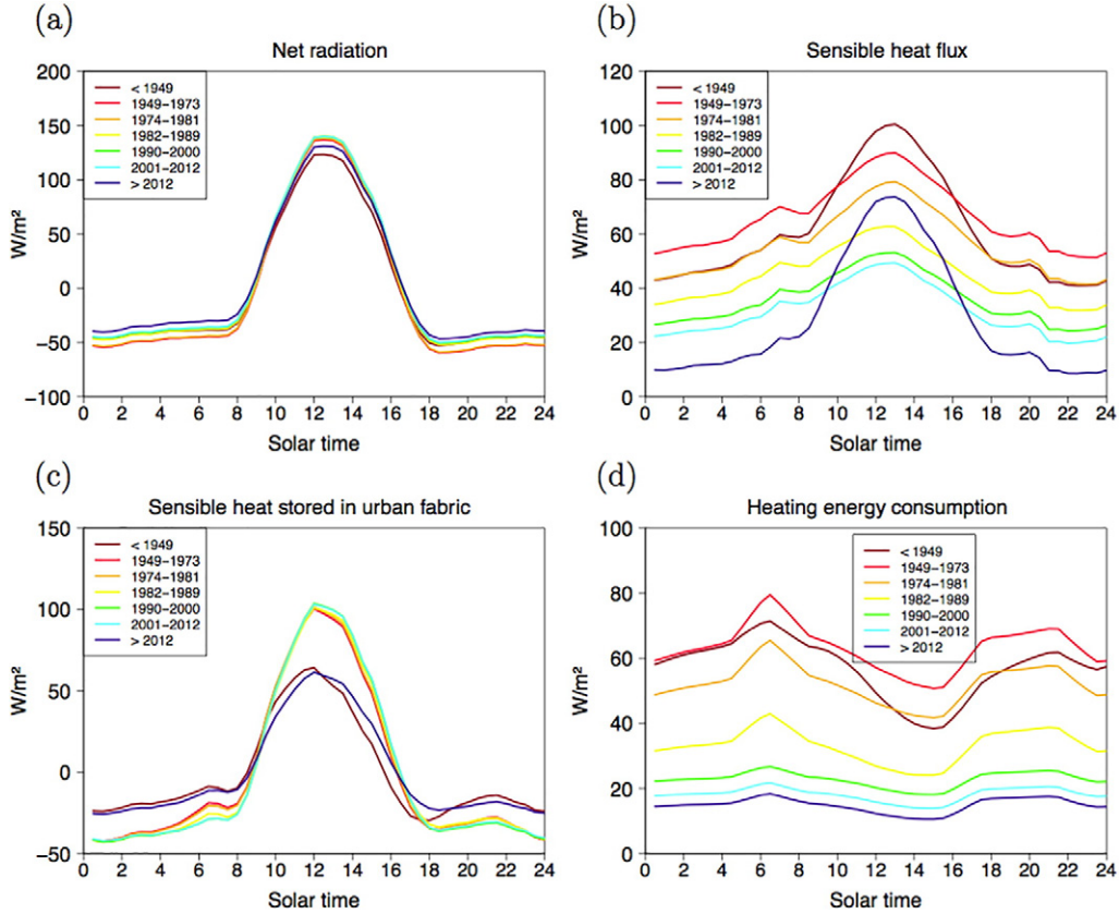
Fig. 7. Sensitivity of the diurnal cycle of (a): net radiation, (b): sensible heat flux, (c): storage heat flux and (d): heating energy consumption on the building construction period. The results are averaged over December, January, February (DJF).
