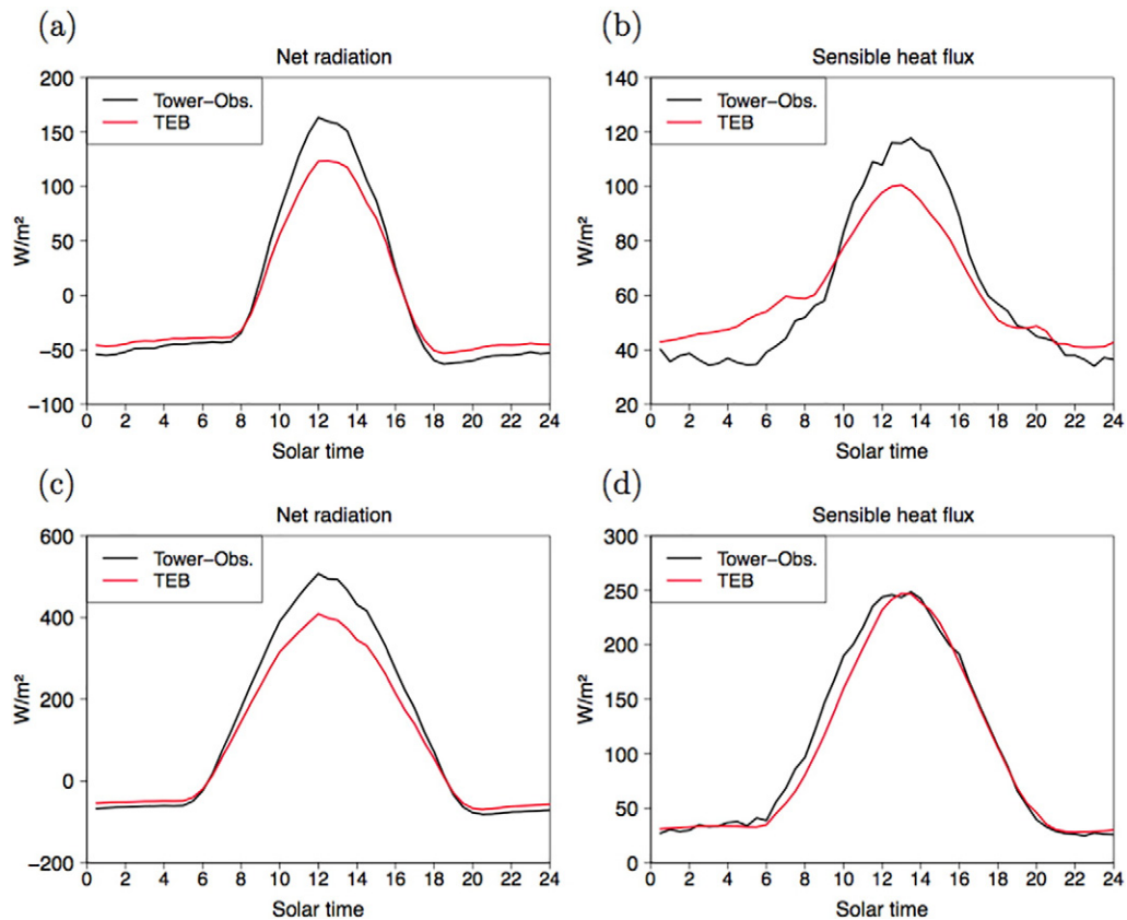
Fig. 8. Comparison between simulated and observed values of (a): net radiation averaged over DJF, (b): sensible heat flux averaged over DJF, (c) and (d): same as (a) and (b), but for JJA. The observed values correspond to the tower observations made during the CAPITOU intensive observation campaign in the centre of Toulouse, France.
