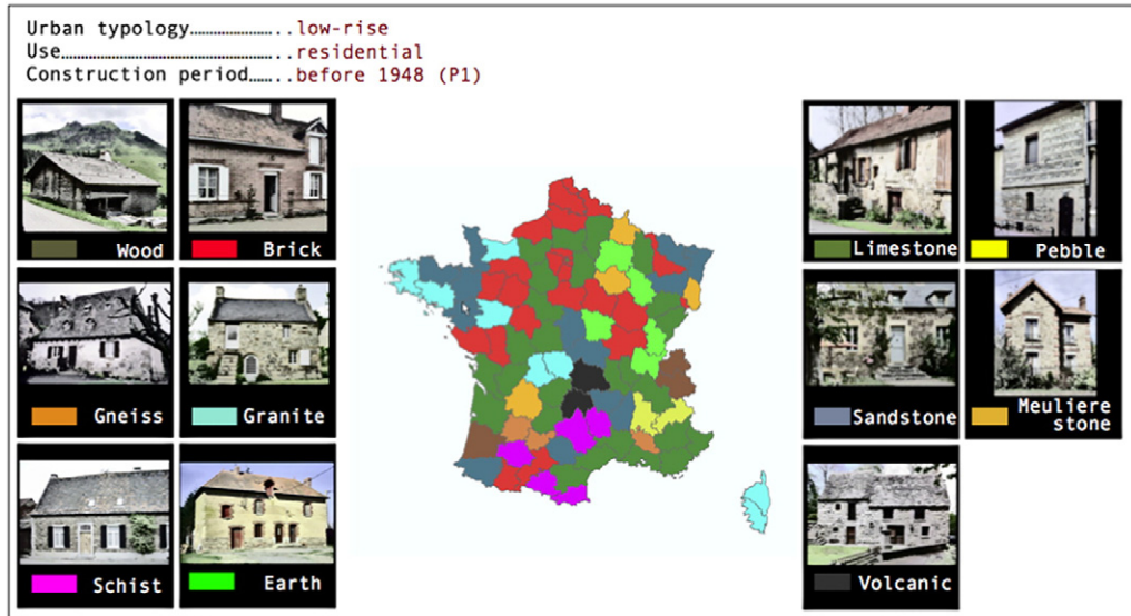
Fig. 3. Geographical distribution of the dominant wall construction material for residential buildings of the French built heritage (P1). The information is available at the scale of a French department.
