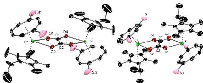
Figure 4: ORTEP diagram of the molecular structure of (8) (left) and (9) (right) with 50% probability ellipsoids. Hydrogen atoms and methyl groups of the \text{SiMe}_3 substituents have been omitted for clarity.
