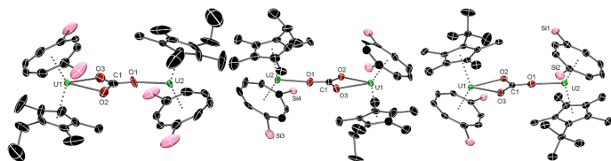
Figure 5: From left to right ORTEP diagrams of the molecular structures of (11), (12) and (13) with 50% probability ellipsoids. Hydrogen atoms and methyl groups of the \text{SiMe}_3 substituents have been omitted for clarity.
