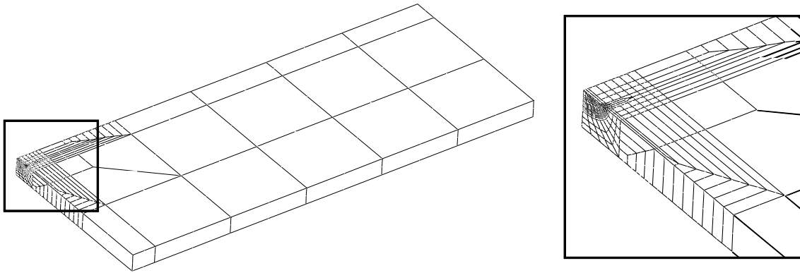
Fig. 3 A solid reference model of the cracked membrane
