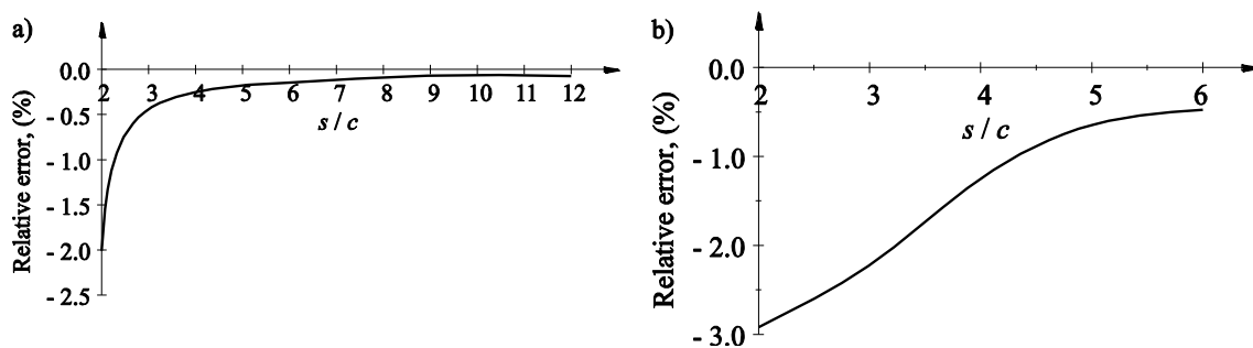
Fig. 8 Dependence of the stress intensity factor on the submodel size:
