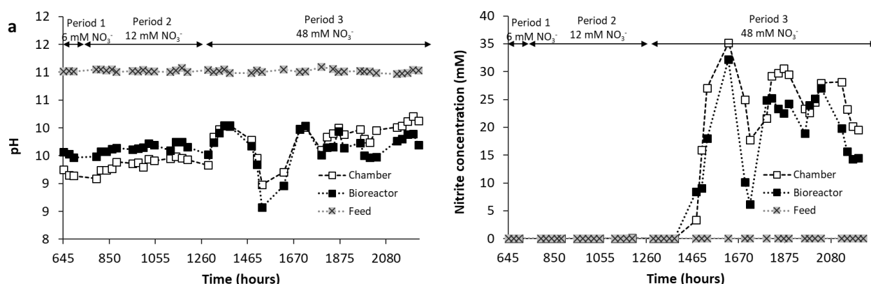
Figure A.3: Microcosm culture under continuous supply with nitrate concentration increasing in the feed solution, nitrate concentration specified in graphics - (a) pH - (b) nitrite concentration in the feed solution ( \times ), the bioreactor ( \blacksquare ) and the exposure chamber ( \square ).
