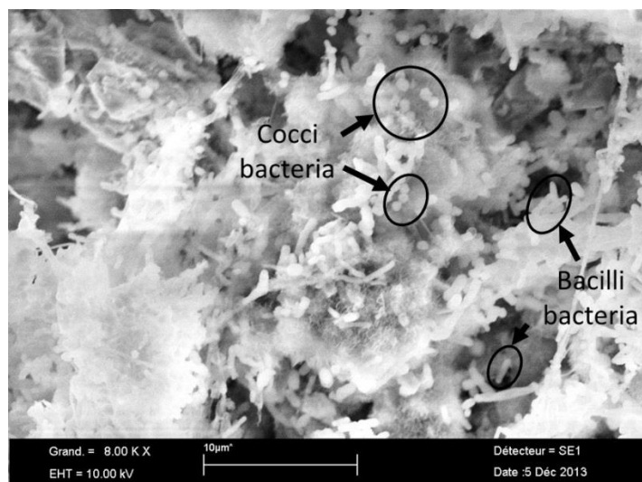
Figure 5: SEM observation of cement paste surface specimen after 700 hours of presence in the culture of the exposure chamber supplied by the bioreactor effluent
