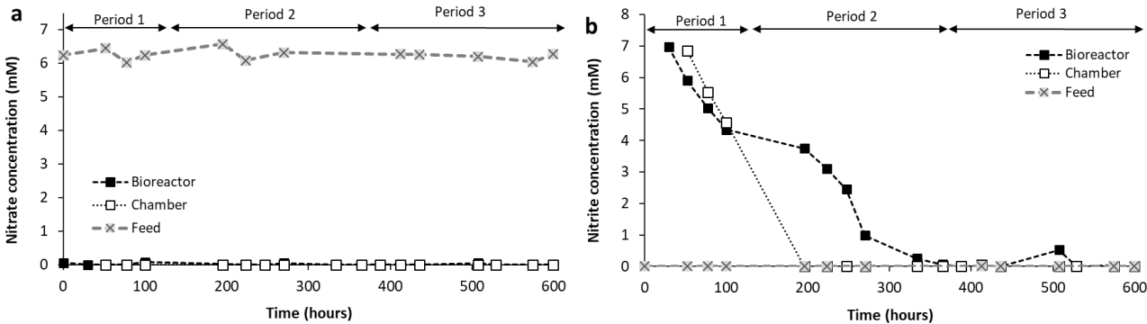
Figure A.2: Microcosm culture under continuous supply and standard condition - (a) nitrate and (b) nitrite concentrations in the feed solution (×), the bioreactor (■) and the exposure chamber (□)
