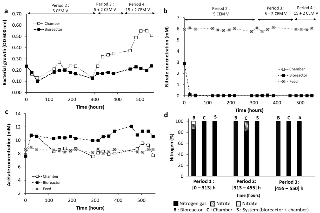
Figure A.5: Continuous culture of sedimentary microcosm at pH 11 with cement paste addition in the exposure chamber - (a) bacterial growth in the bioreactor and exposure chamber, (b) nitrate concentration, (c) acetate concentration in the feed solution (x), the bioreactor (■) and the exposure chamber (□) - (d) nitrogen mass balance on the bioreactor, the chamber and on the system (i.e. bioreactor + chamber)
