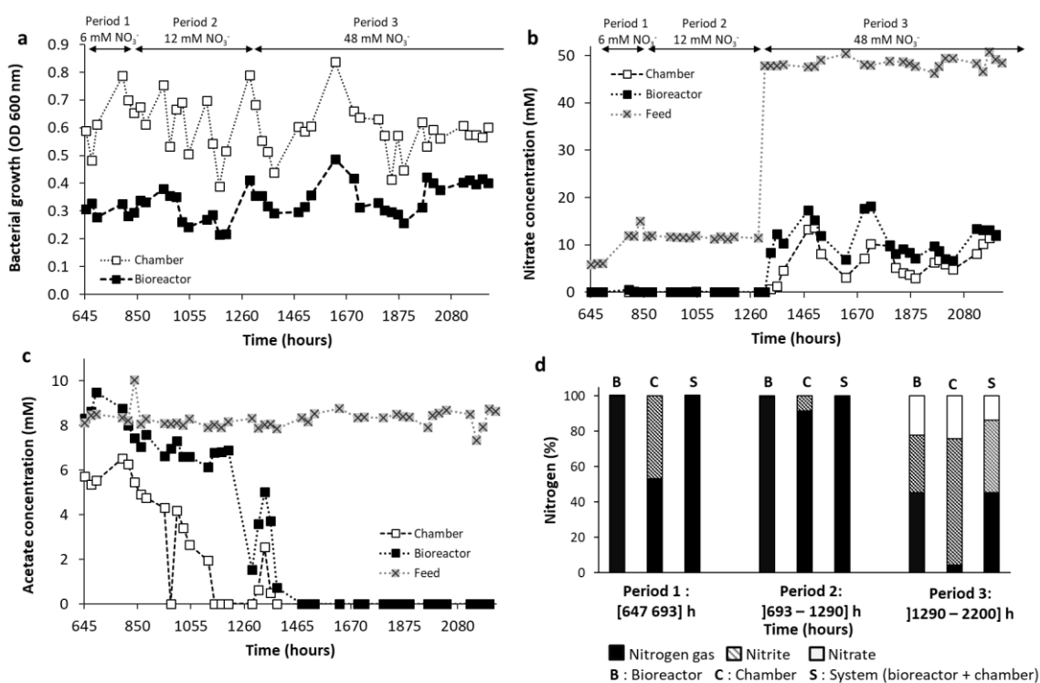
Figure 6: Monitoring of the microcosm culture under continuous supply of standard medium with nitrate concentration increasing from 6.0 to 48 mM – (a) bacterial growth, (b) nitrate concentration, (c) acetate concentration; in the feed solution (×), the bioreactor (■) and the exposure chamber (□) - (d) nitrogen mass balance: in the bioreactor, the chamber and the complete system (i.e. bioreactor + chamber)
