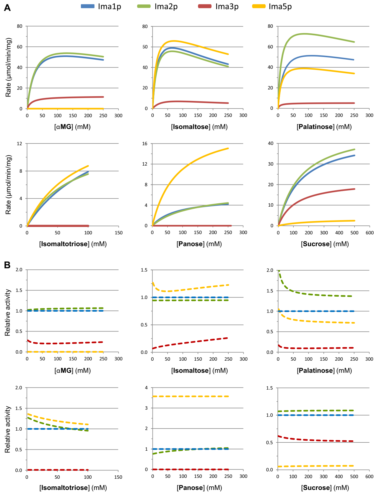
Fig. 2. Overview of Velocity-Substrate profiles and relative activities. Comparative plots of the four isomaltases (Ima1p, blue; Ima2p, green; Ima3p, red; Ima5p, yellow) on different substrates (α-MG, isomaltose, palatinose, isomaltotriose, panose and sucrose, respectively). (A) Representative curves of the velocity as a function of substrate concentration, plotted from the equation: v = (V_{\max} S)/(K_m + S(1 + S/K_i)) . For each isomaltase/substrate pair, V_{\max} , K_m and K_i values can be found on the original plots (Fig. 1 and Fig. S4A–D). (B) Overview of relative activities, where the ratio of velocities ( v_{\text{Imaxp}}/v_{\text{Ima1p}} , Ima1p being taken as the reference) is plotted as a function of substrate concentration. (For interpretation of the references to colour in this figure legend, the reader is referred to the web version of this article.)
