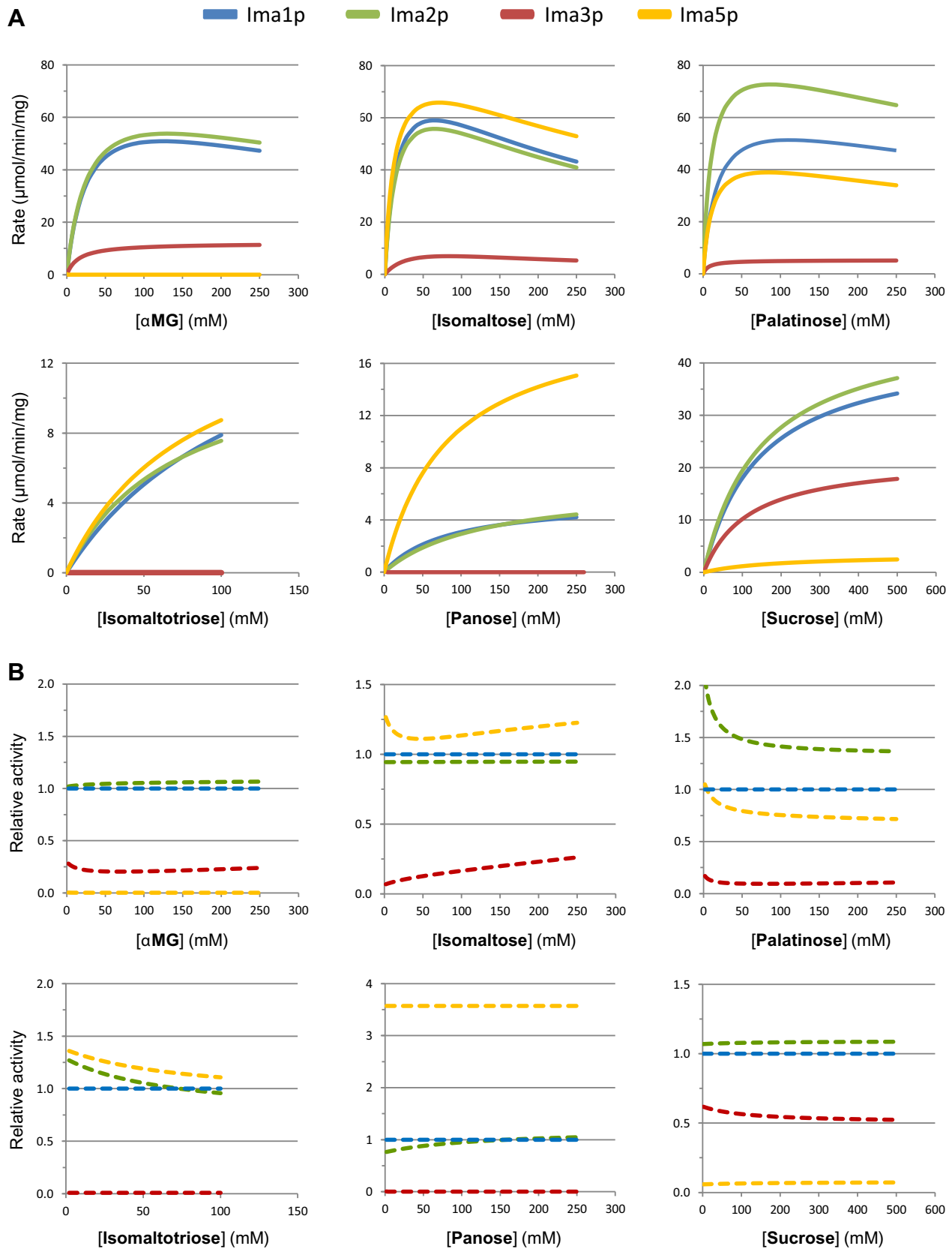
Fig. 2. Overview of Velocity-Substrate profiles and relative activities. Comparative plots of the four isomaltases (Ima1p, blue; Ima2p, green; Ima3p, red; Ima5p, yellow) on different substrates (α-MG, isomaltose, palatinose, isomaltotriose, panose and sucrose, respectively). (A) Representative curves of the velocity as a function of substrate concentration, plotted from the equation: v = (V_{\max} S) / (K_m + S(1 + S/K_i)) . For each isomaltase/substrate pair, V_{\max} , K_m and K_i values can be found on the original plots (Fig. 1 and Fig. S4A–D). (B) Overview of relative activities, where the ratio of velocities ( v_{\text{Imaxp}}/v_{\text{Ima1p}} , Ima1p being taken as the reference) is plotted as a function of substrate concentration. (For interpretation of the references to colour in this figure legend, the reader is referred to the web version of this article.)
