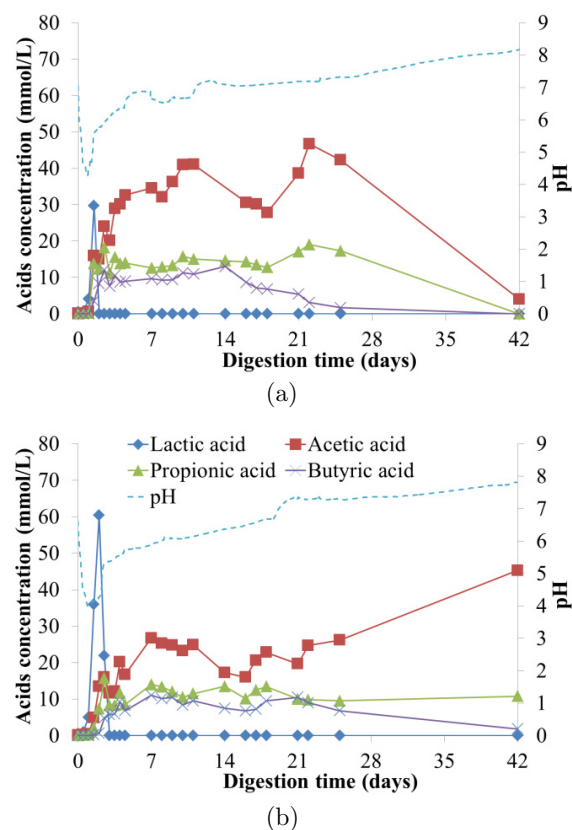
Fig. 3. Concentration of acids and pH during the anaerobic digestion of biowaste in presence (a) and in absence (b) of ordinary cement paste sample in the bioreactors.
