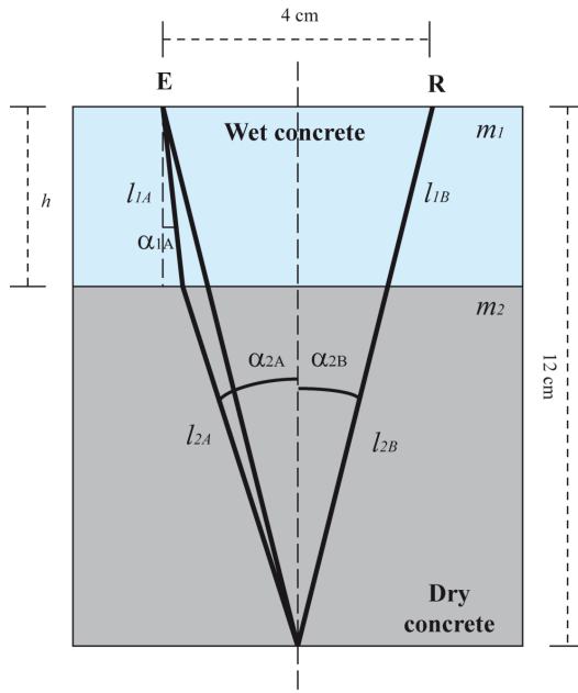
Figure A1. Electromagnetic traveling paths models.
