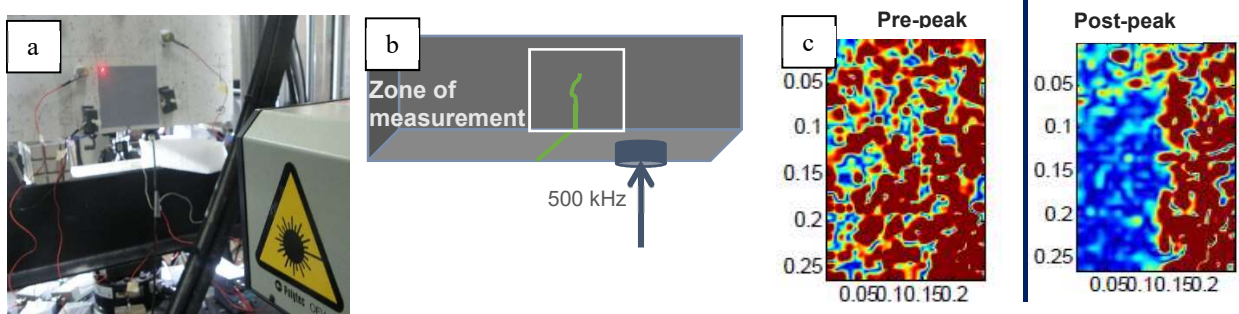
FIGURE 7. a) Us antenna measurement b) Principle c) Maps of diffused waves before and after the peak.
