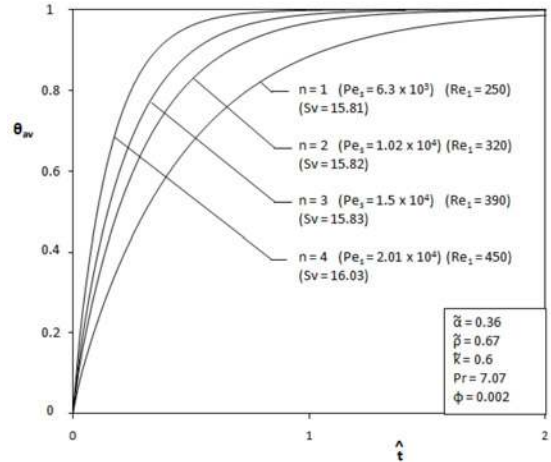
Figure 5 The effect of complexity ( n ) on the evolution of the system average temperature in a three-dimensional configuration [13].
