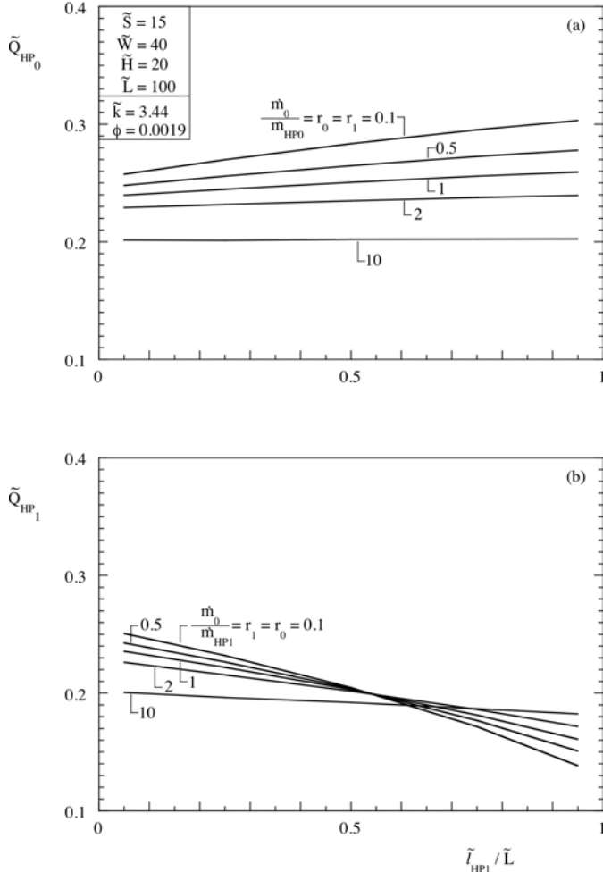
Figure 11 The variation of the dimensionless enthalpy gain of the (a) HP_0 and (b) HP_1 with the connection position l/\tilde{L} of the HP_1 and the equal ratios between the mass flow rates ( S/D = 15 , \phi = 0.0019 , L/D = 100 , W/D = 40 , H/D = 20 ) [16].
