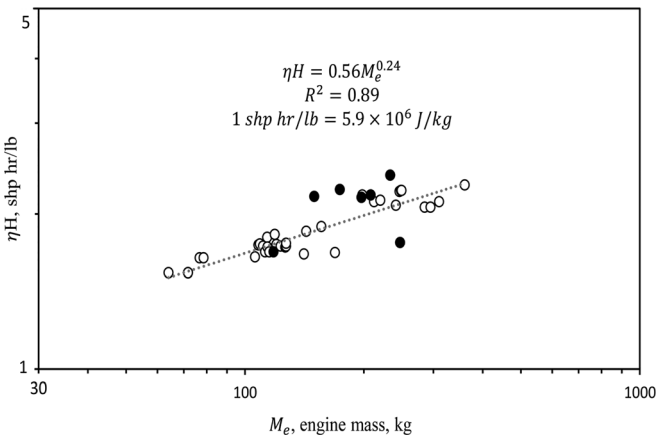
FIG. 5. The correlation between helicopter engine efficiency and engine size. In the indicated correlation, the military helicopter data (the black circles) were not included. If the military data are included, the correlation becomes \eta H = 0.53M_e^{0.25} , with R^2 = 0.79 . 22
