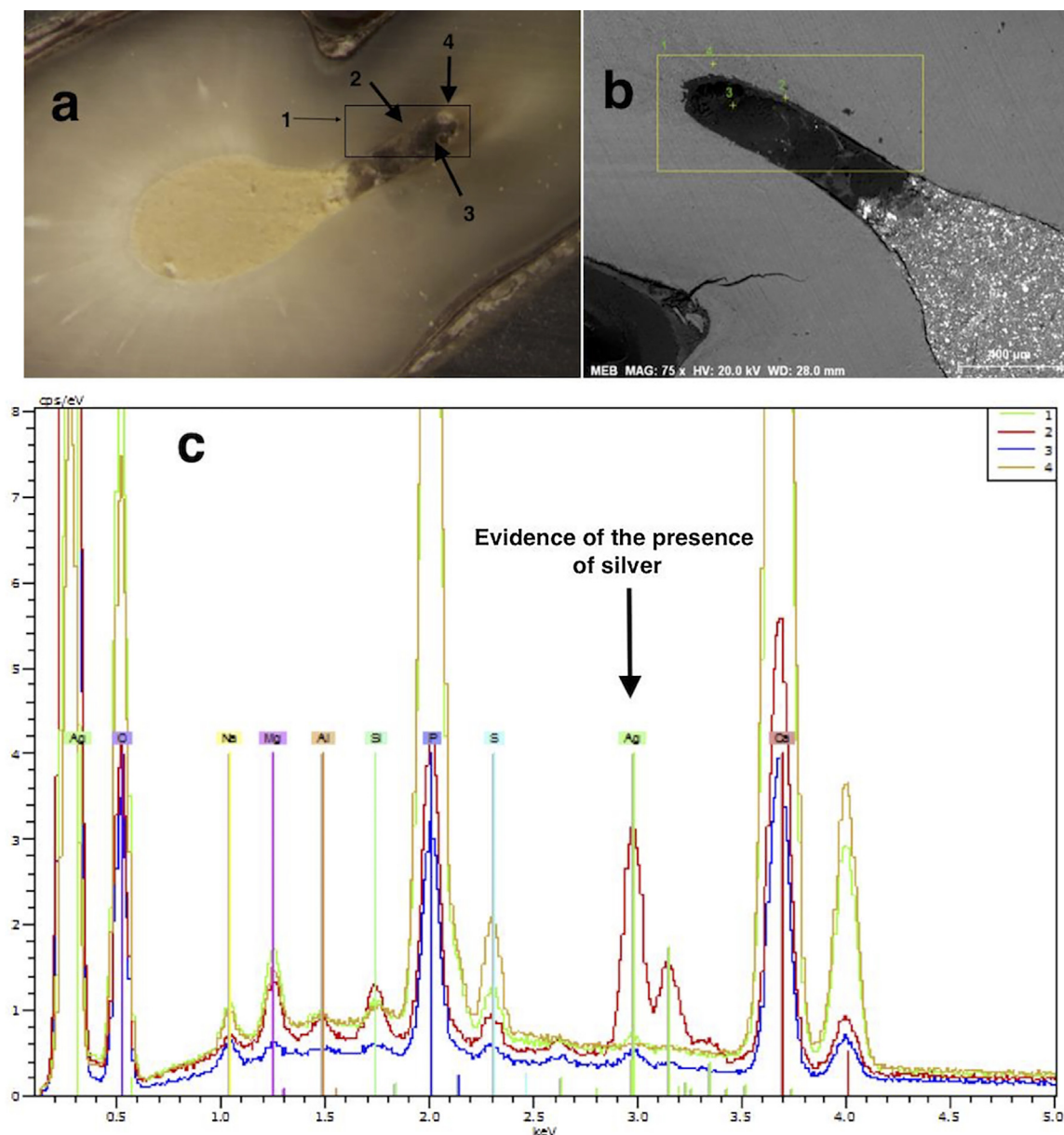
Figure 4 Scanning Electron Microscope analysis of this slice. (a) Choosing a zone of interest 1 and multiple points 2, 3, 4. (b) Choosing the same points on the SEM image. (c) Energy Dispersion Spectroscopy EDS of these points indicates the presence of Silver at least with point 2.
