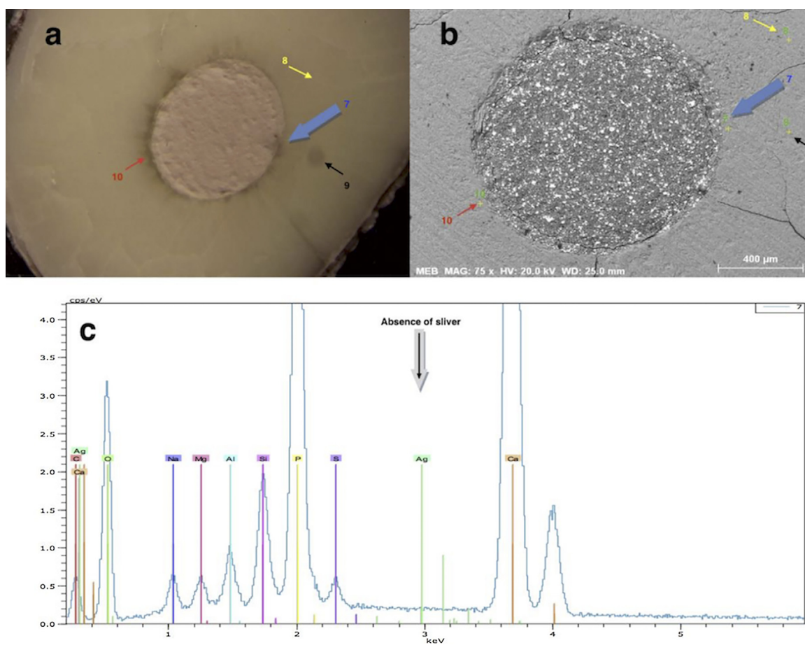
Figure 3 Scanning Electron Microscope analysis of this slice. (a) Choosing multiple points of interest. (b) Choosing the same points on the SEM image. (c) Energy Dispersion Spectroscopy EDS of the point n°7 indicates the absence of the dye in this point. The same procedure was repeated for all points of interest and the final score given to this slice was 0 due to the absence.
