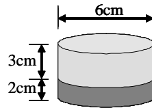
Fig. 19 – Specimen dimensions used to characterize the Coulomb model
