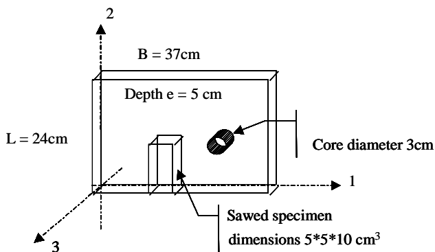
Fig. 3 – Brick and sample dimensions
